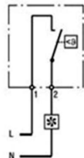
Thermostat KTS 011 (NO)
