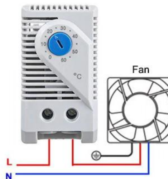
KTS 011(NO.) Cooling
